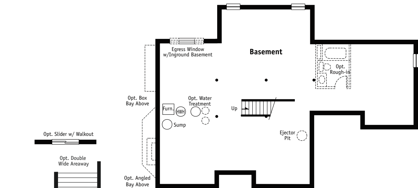
Unfinished Basement Plan (Not to Scale)
