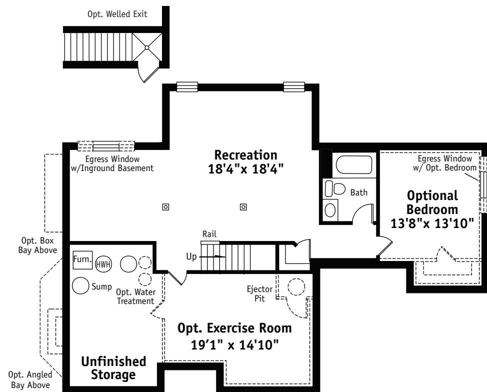
Opt. Finished Basement Plan (Not to Scale)
