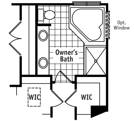
Partial Plan w/Opt. Alt. Bath
