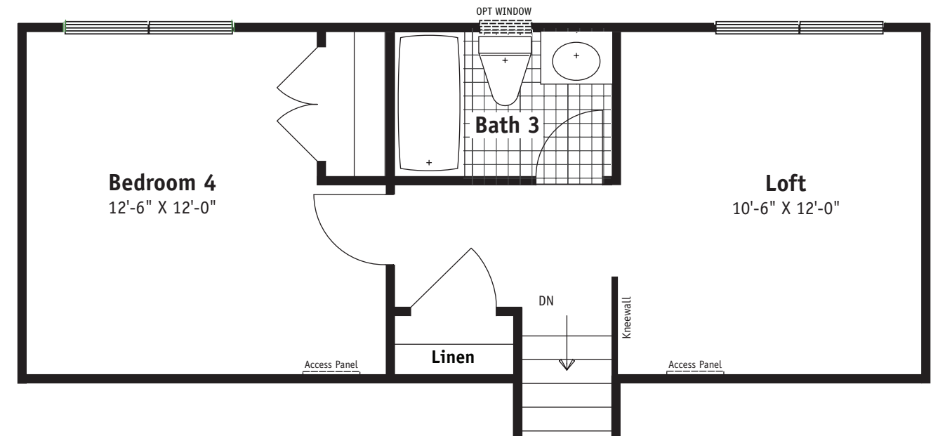
Optional Third Floor Loft Plan
