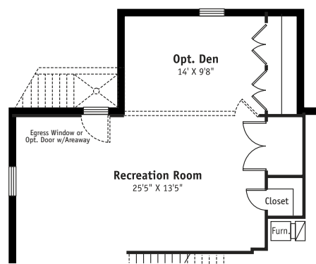
Finished Basement w/Optional Morning Room
