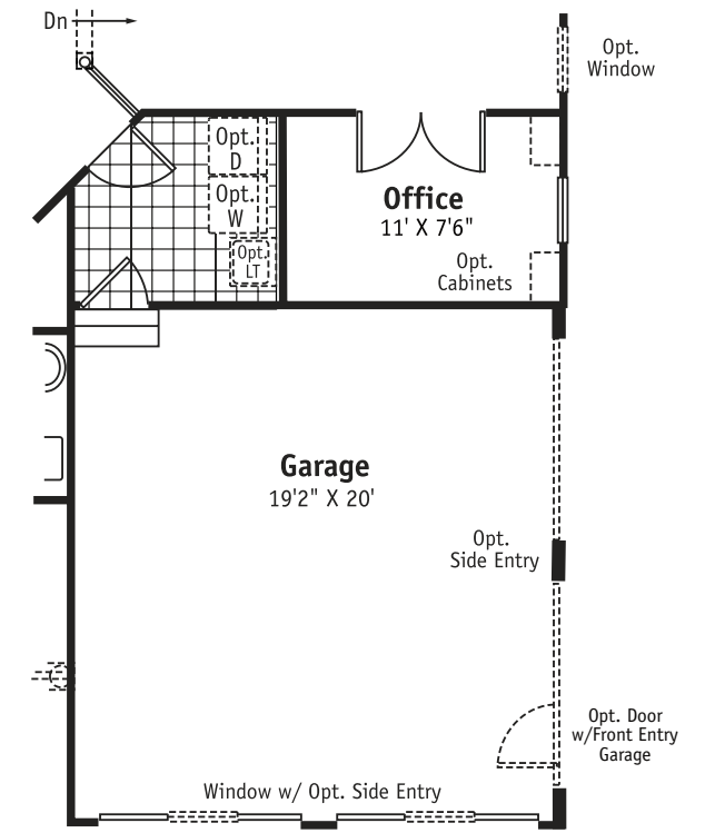
Opt. Home Office - Partial Plan
