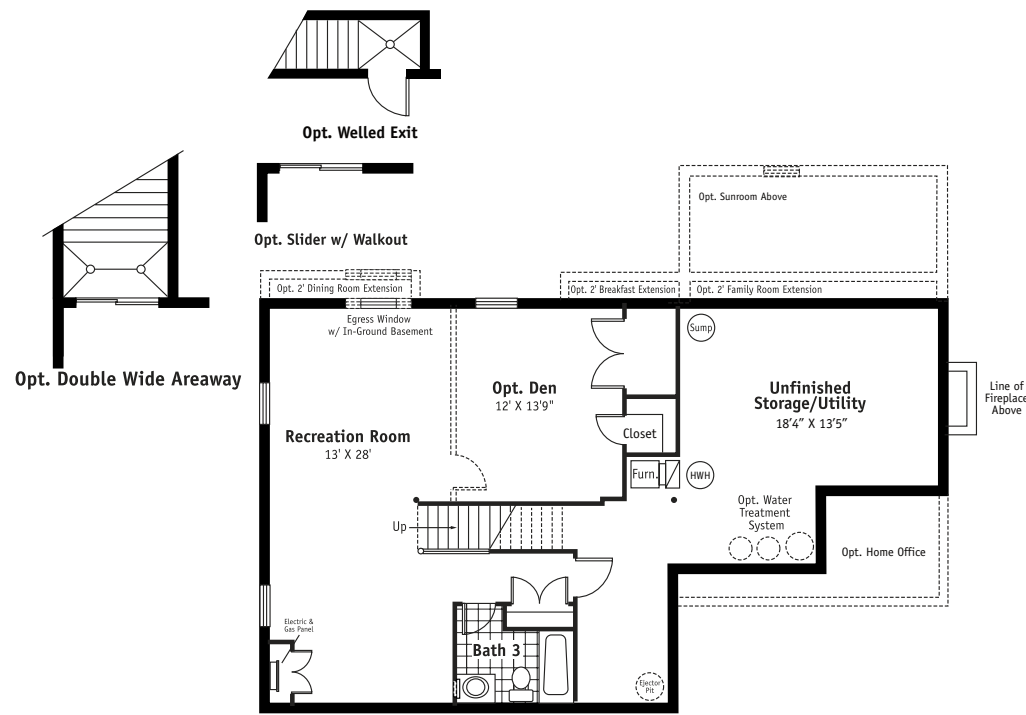
Opt. Finished Basement
