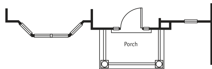
First Floor Plan/Elev. 2 - Partial Plan
