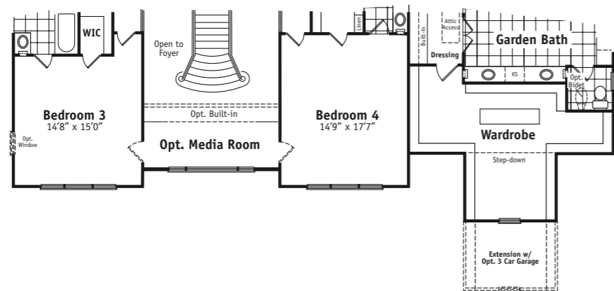
Partial 2nd Floor Plan w/Elev. 3
