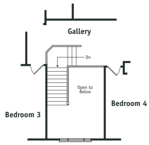
Partial Second Floor Plan w/Alternate Staircase
