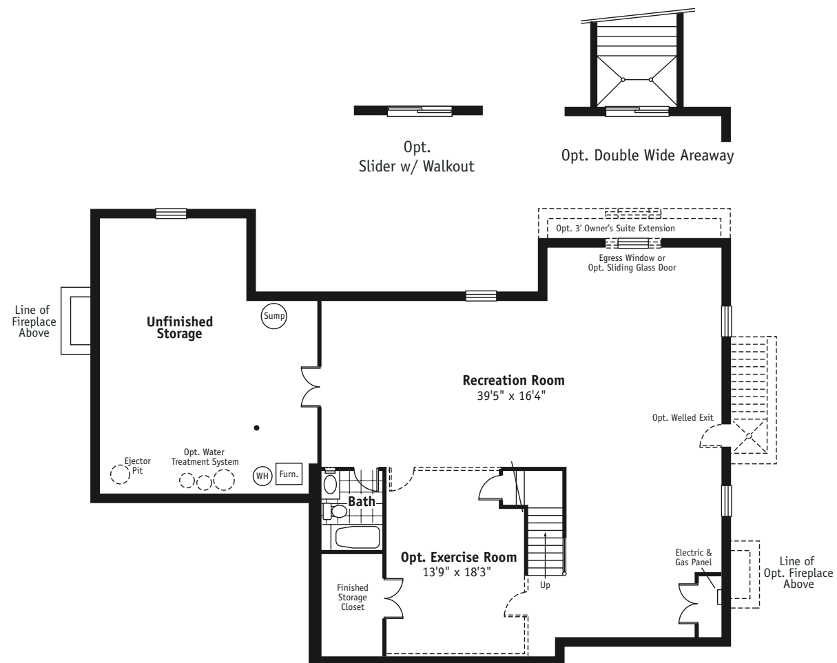
Unfinished Basement Plan
