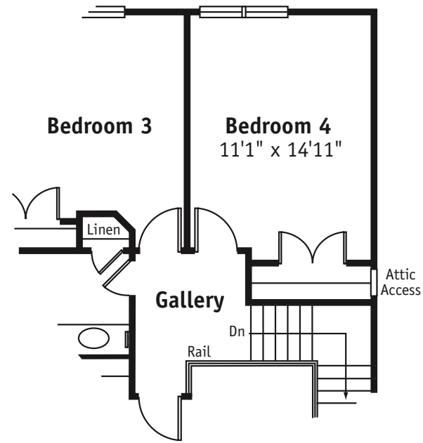
Partial Plan: Bedroom 4 ILO/Loft
