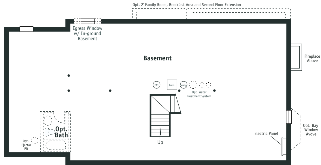
Unfinished Basement Plan
