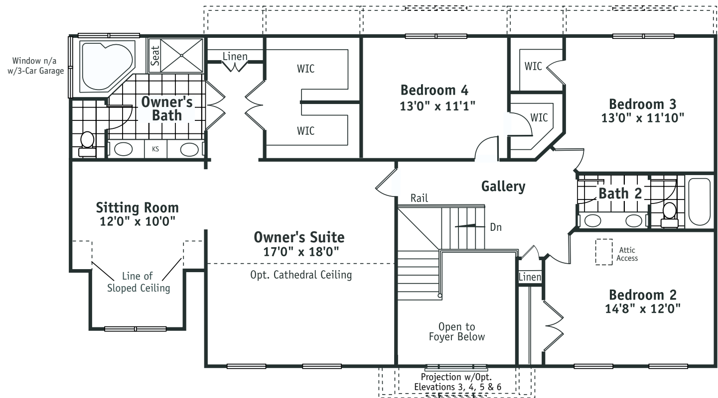
Optional Second Floor Plan-A
