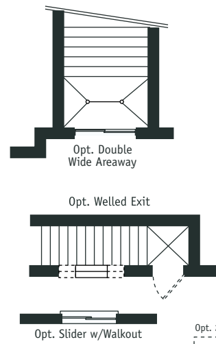
Unfinished Basement Plan
