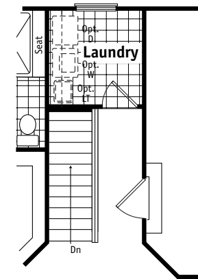
First Floor Plan w/Opt. Fin. Basement
