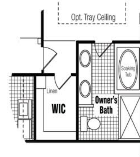
Partial Plan w/Opt. Alternate Bath
