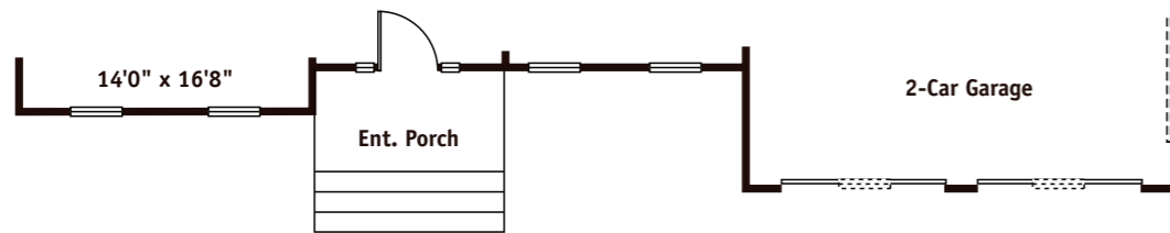
Partial First Floor Plan w/Elev. 4
