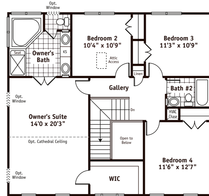
Standard Second Floor Plan
