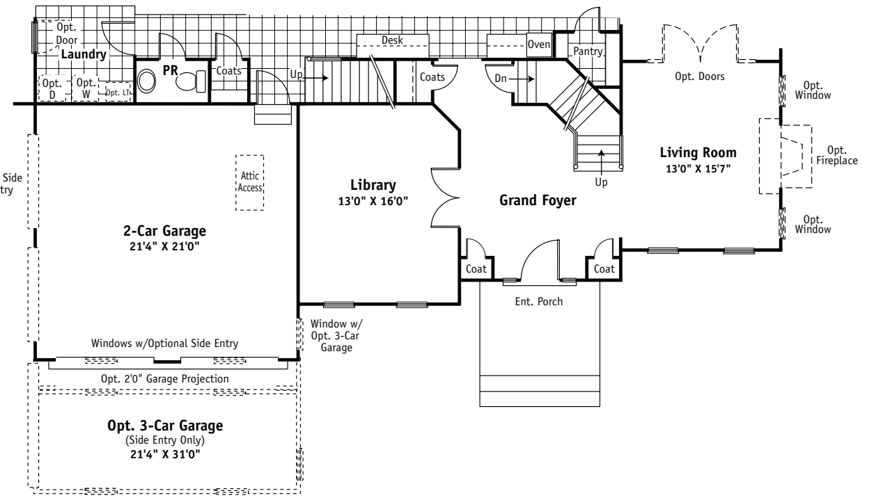
Partial First Floor Plan w/Elevation #5
