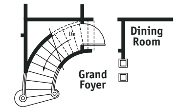
Partial Plan w/Curved Stair
