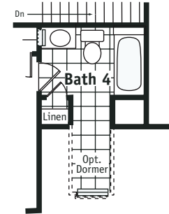
Partial Plan w/Bath 4 and Opt. Active Dormer
