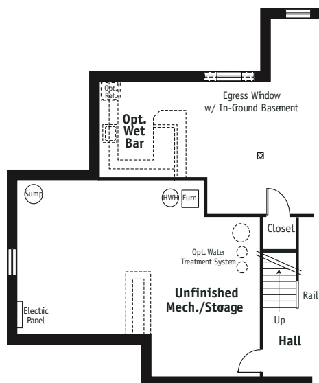
Partial Finished Basement Plan w/ Opt. Sunroom
