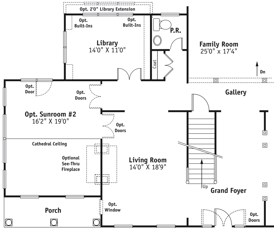
Partial First Floor Plan W/ Optional Sunroom #2
